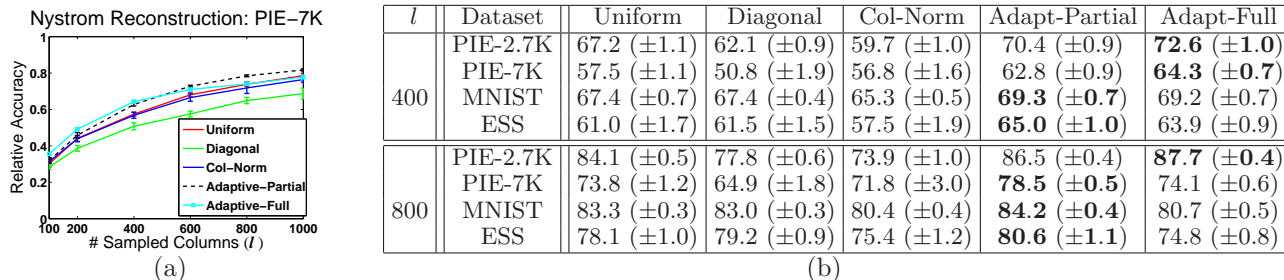
Figure 4. Nyström spectral reconstruction accuracy for various sampling methods for k = 100 . (a) Results for PIE-7K using several values of l . (b) Results for all datasets for two values of l with k = 100 . Numbers in parenthesis indicate the standard deviations for 10 different runs for each l .
