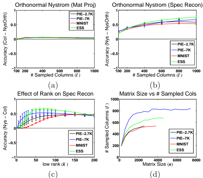
Figure 2. (a) Difference in matrix projection between Column-sampling and Orthonormal Nyström ( k = 100 ). Values above zero indicate better performance of Column-sampling. (b) Difference in spectral reconstruction between Nyström and Orthonormal Nyström ( k = 100 ). Values above zero indicate better performance of Nyström method. (c) Difference in spectral reconstruction accuracy between Nyström and Column-sampling for various k and fixed l = 600 . Values above zero indicate better performance of Nyström method. (d) Number of columns needed to achieve 75% relative accuracy for Nyström spectral reconstruction as a function of n .
